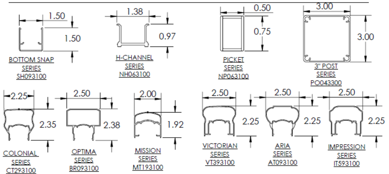
FIGURE 1—TYPICAL GUARDRAIL ASSEMBLY AND COMPONENT PROFILES
